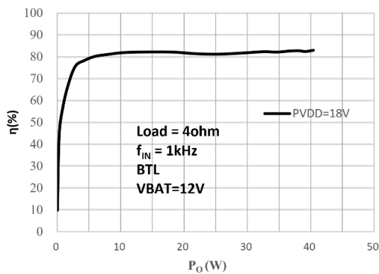
P_O vs \eta
