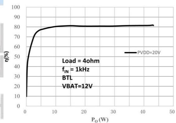
P_O vs \eta
