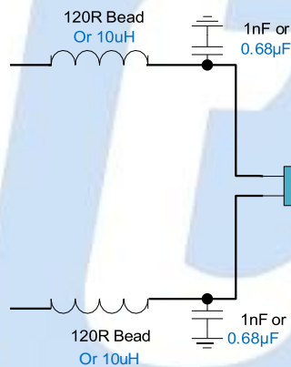
Figure 3 Output Filters Configurations
