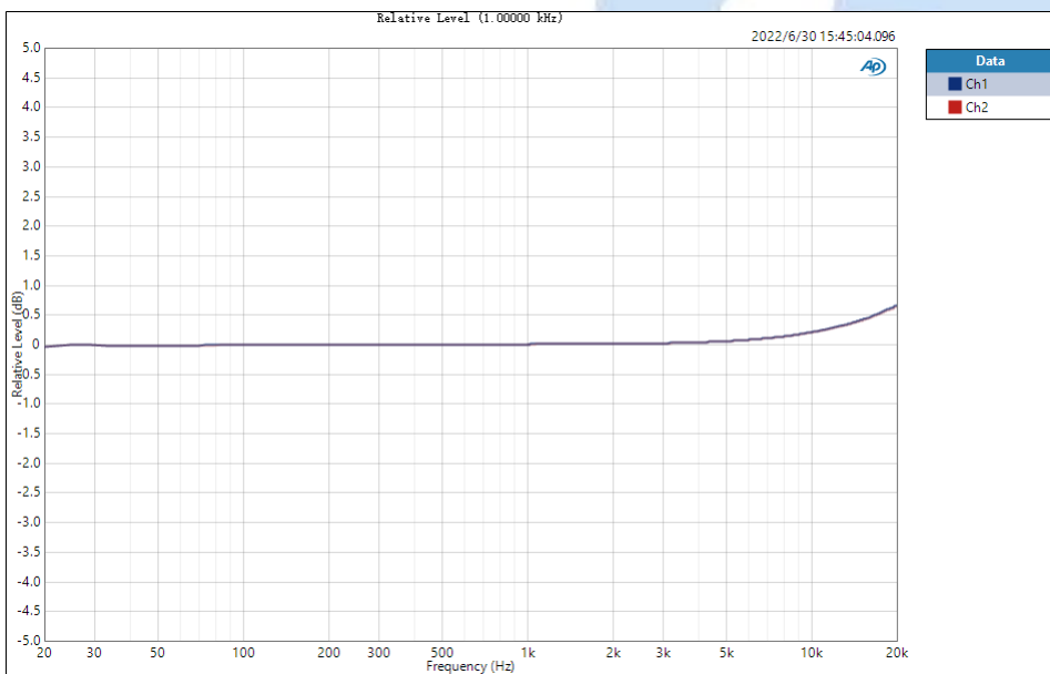
Frequency respond (Cin = 1uF, Rin=0k, Gain=L)
