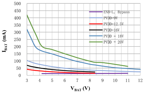
Quiescent Current
