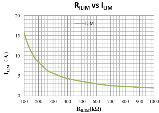
Figure 1 Peak Current Limit (I LIM ) vs I LIM terminal resistor (R LIM )
