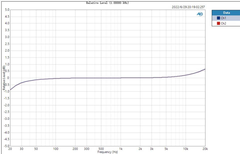
Frequency respond (Cin = 1uF, Rin=10k, Gain=H)
