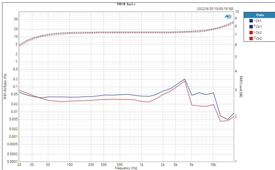
frequency vs THD+N ( P_o \approx 2 \times 7.5W )
